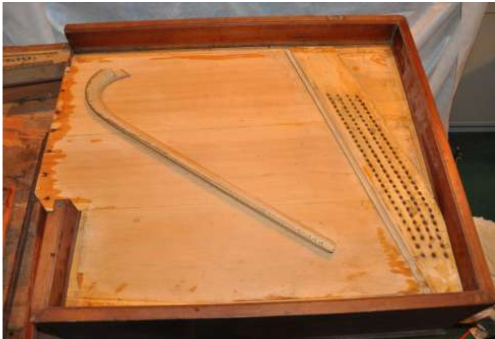
Molding up, ready to re-apply towels directly to soundboard joints
